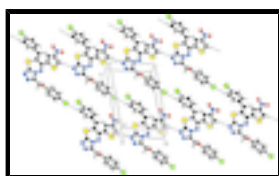
Fig. 2. The crystal packing of the title compound, viewed along the a axis. Hydrogen bonds are shown as dashed lines.
